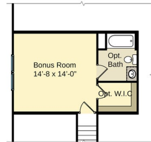
Second Floor Plan 1/4" = 1'-0" (OPTIONAL BONUS w/ BATH)
