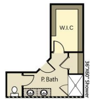
Primary Bath Shower Layout Option 1
