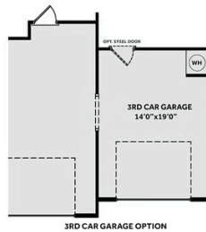
3RD CAR GARAGE OPTION
