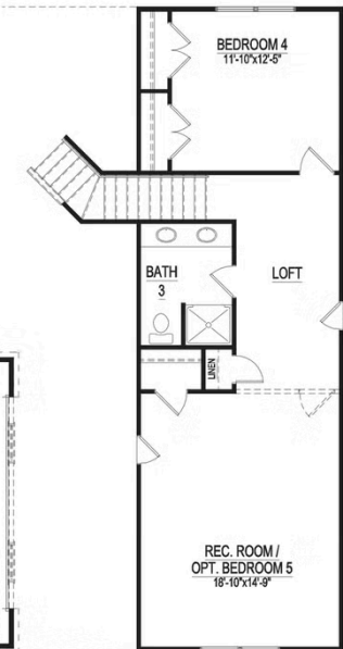
OPT. SECOND FLOOR PLAN
