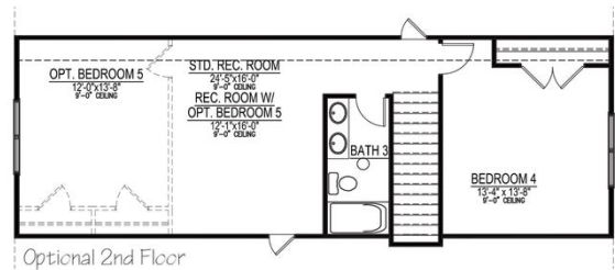
Optional 2nd Floor
